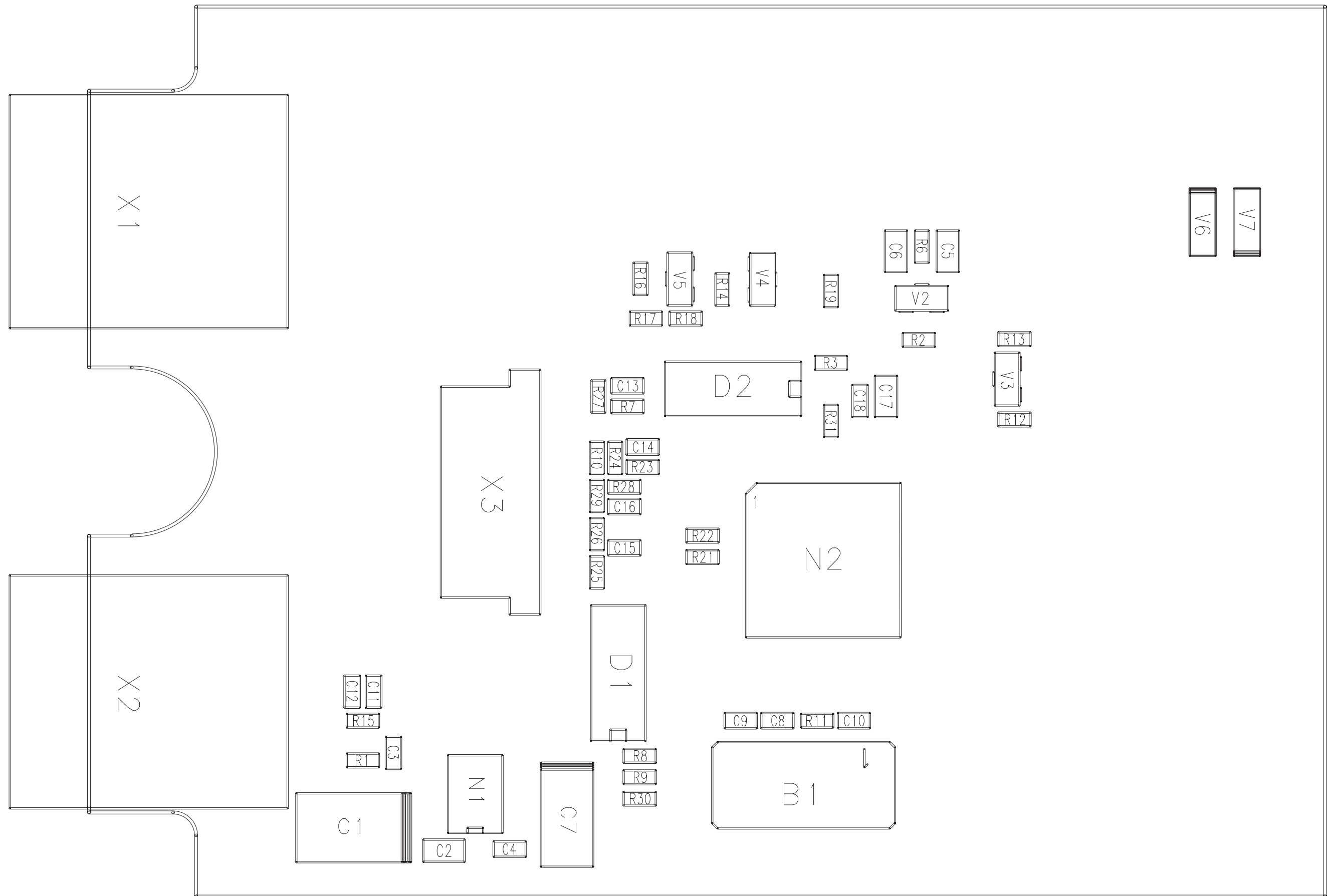
Figure 4: Component Layout Diagram of GM8S
